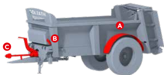
(A) Steel mudguards (B) Document tube with individualised spare parts book (C) Hose holder and wide-angle P.T.O.-shaft with cam security.
