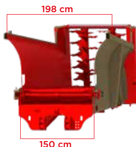
Rounded body to facilitate the unloading of goods, made by bending the sheet metal for an increased rigidity of the side walls.
